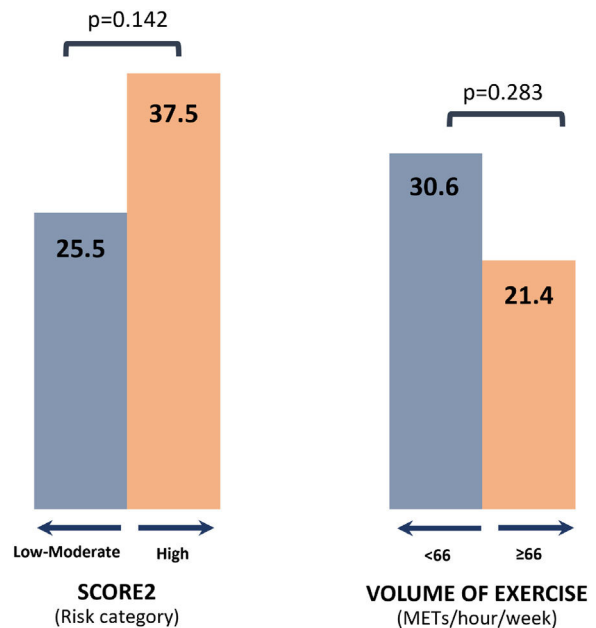
Figure 1 Proportion of individuals with high coronary atherosclerotic burden across the categories of CV risk and volume of exercise.
