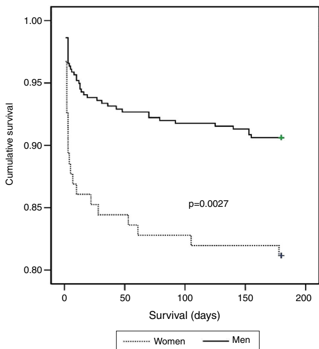
Figure 1 Survival function.
